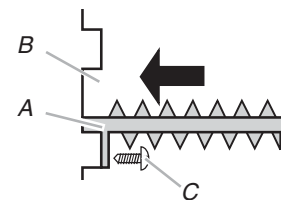
A. Side curtain against window channel B. Window channel C. #8 x \frac{3}{4} " round-head screw
